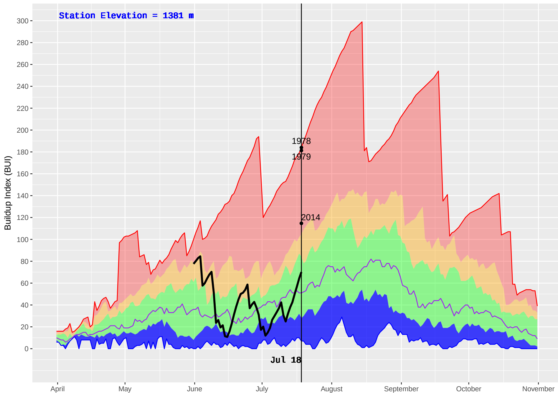
GLIMPSE (291) : Historical (1978–2016) and Current (2018) Daily Buildup Index (BUI)
